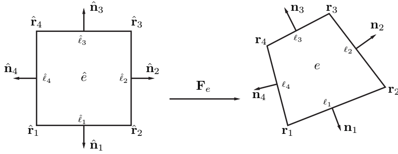
FIG. 2.2. Bilinear mapping and orientation of normal vectors.
