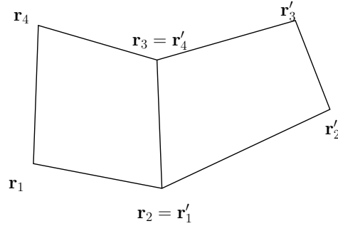
FIG. 2.1. h^2 -uniform quadrilateral grid.
