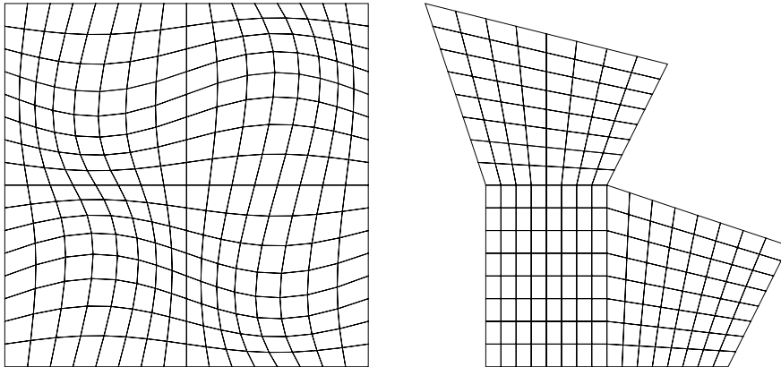
FIG. 6.1. Examples of meshes used in numerical experiments.
