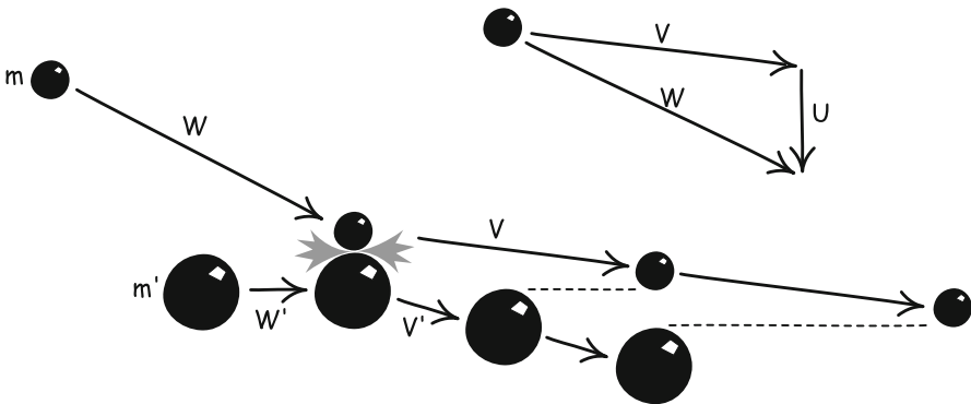
Fig. 2 Hard body collision
