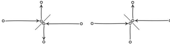
Figure 6. Resolving collisions.
