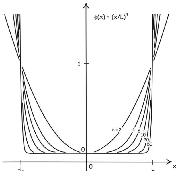
Figure 8. Analytic potential functions approach nonanalytic limit.
