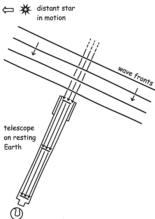
Figure 2.15. Lorentz transformation of Figure 2.13 to a resting Earth.
