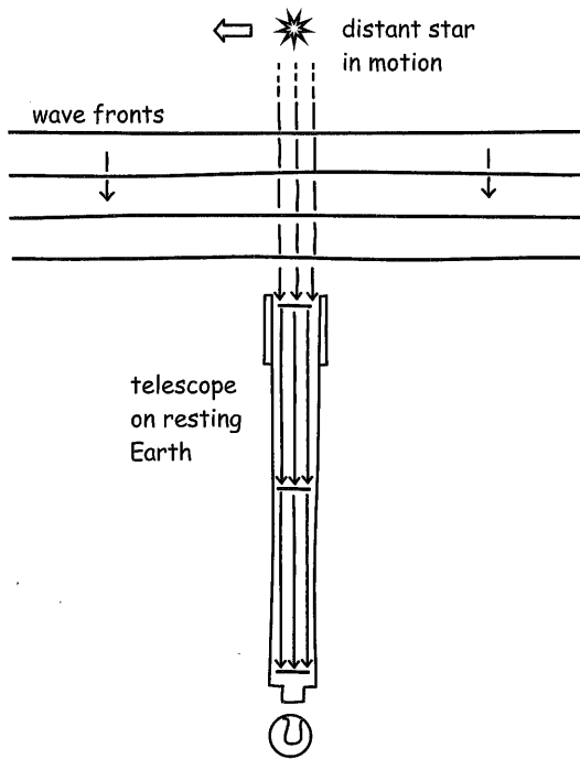
Figure 2.14. Galilean transformation of Figure 2.13 to a resting Earth.
