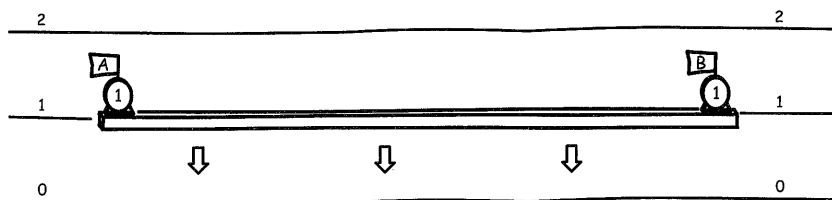
Figure 2.3. Vertical motion.
