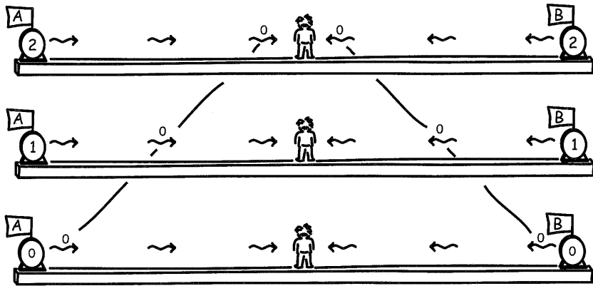
Figure 2.1. Checking the synchrony of two clocks.
