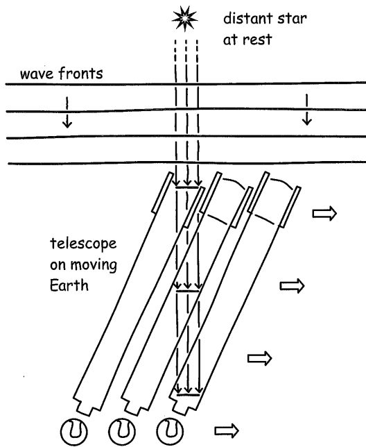
Figure 2.13. Stellar aberration in an ether-based wave theory of light.
