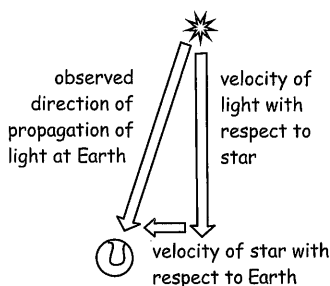
Figure 2.12. Stellar aberration.
