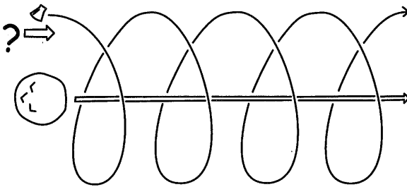
Figure 2.6. A hard problem in Newtonian physics .
