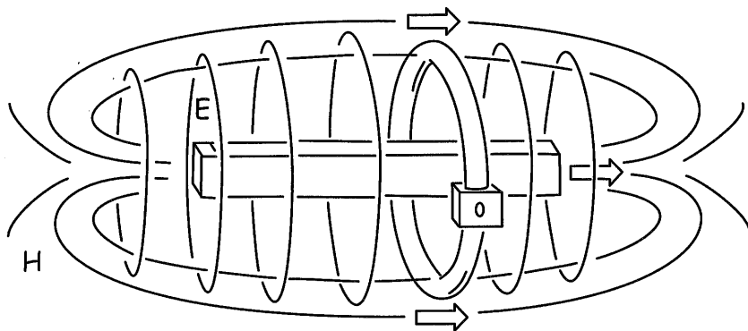
Figure 2.9. Magnet and conductor moving in the ether.
