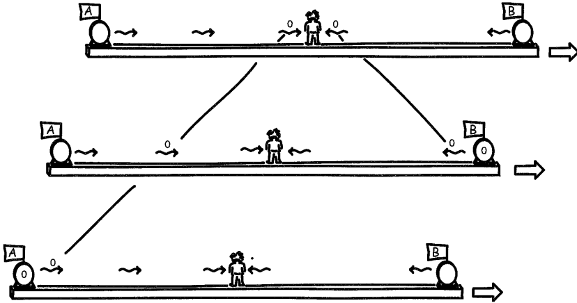
Figure 2.2. Check of clock synchrony as seen by a moving observer.
