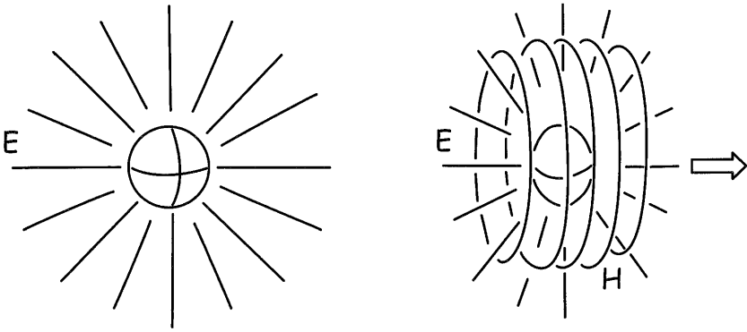
Figure 2.5. Lorentz's electron at rest and in motion .
