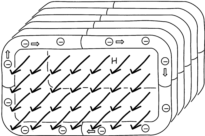
Figure 2.10. Magnetic field inside a coil as seen by a comoving observer.
