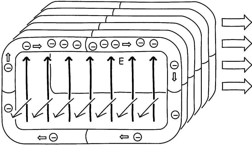
Figure 2.11. Induced electric field inside a moving coil.
