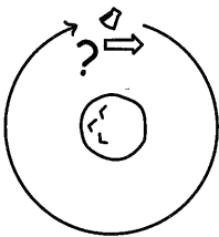
Figure 2.7. An easy problem in Newtonian physics .
