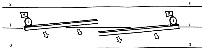
Figure 2.4. Vertical motion seen by a horizontally moving observer.
