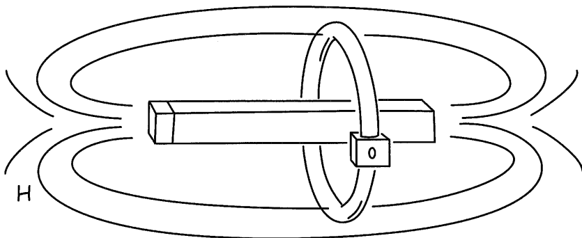
Figure 2.8. Magnet and conductor at rest in the ether.
