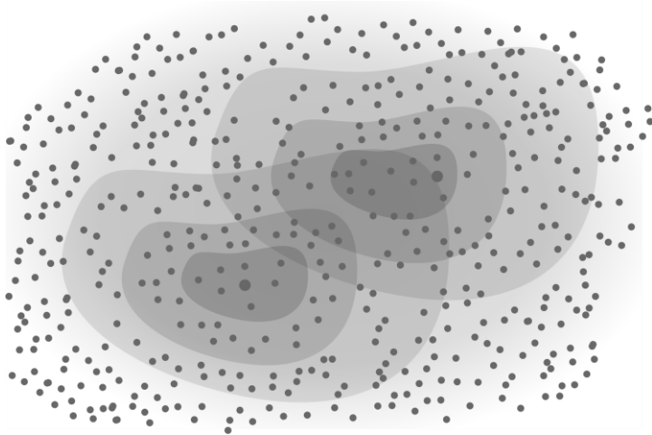
Figure 3 A manifold of spacetime events.
