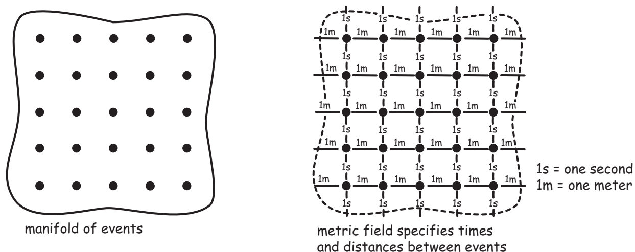
Figure 6. Manifold and Metric
