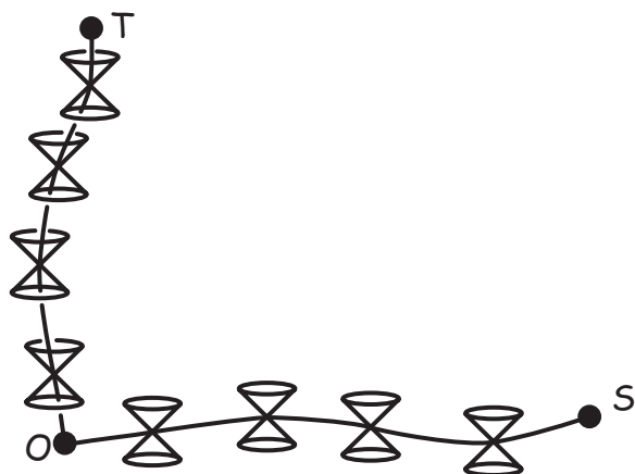
Figure 9. Causal Connectivity
