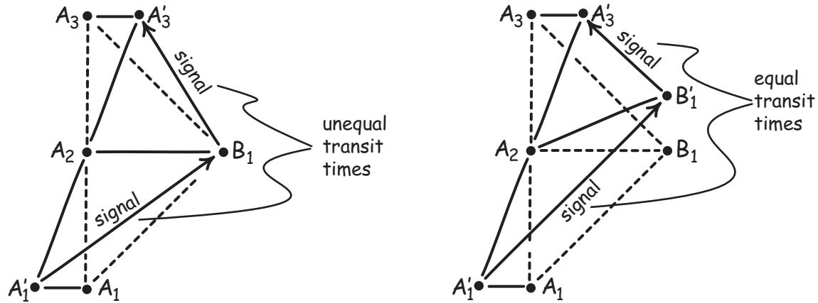
Figure 15. In Relativistic spacetimes, different inertial observers can disagree on which pairs of event are simultaneous.
