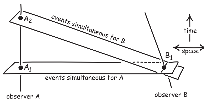
Figure 5. Determinateness of the future?
