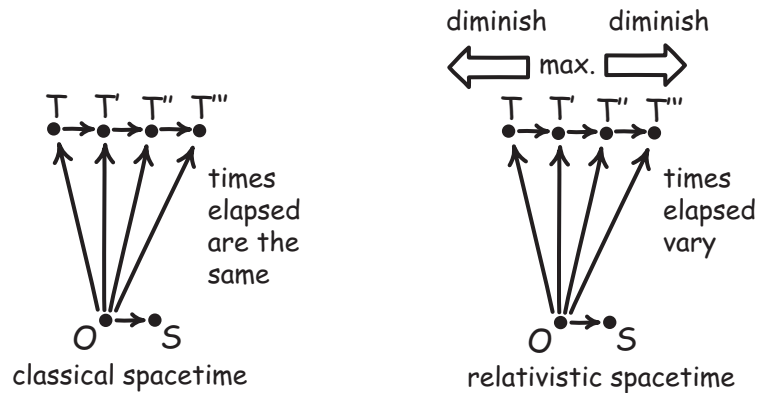
Figure 4. Entanglement of time and space in relativistic spacetimes.
