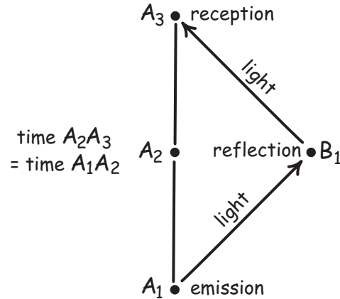
Figure 13. Events A_2 and B_1 are simultaneous by Einstein's Definition
