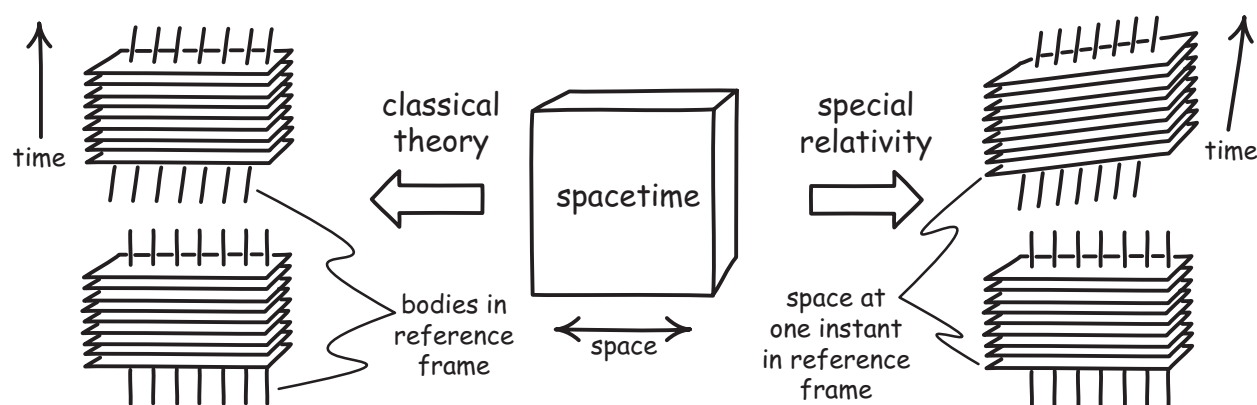
Figure 1. Simultaneity in classical theory and special relativity
