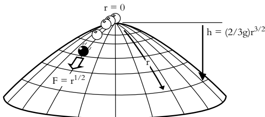
Figure 2.1a. Mass sliding on a dome.
