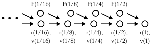
Figure 2.8. An infinite chain of causes with no first cause.
