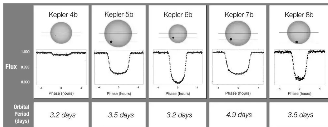
Figure 12. Brightness dip from exoplanet transit 16
