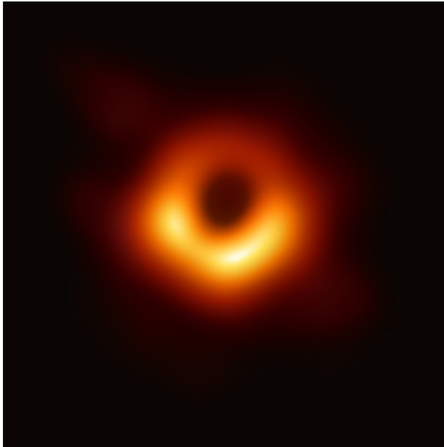
Figure 13. Event Horizon Telescope image of the black hole in galaxy M87 18
