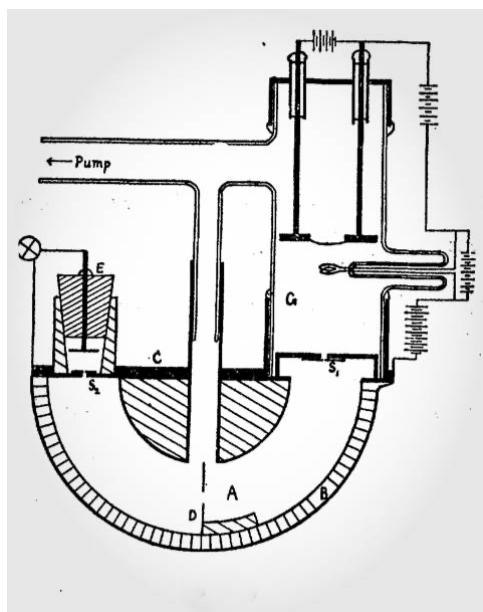
Figure 7. Dempster's mass spectrometer 11
