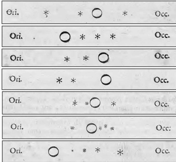
Figure 10. Galileo's first seven images of Jupiter and its surrounding moons on successive nights 14
