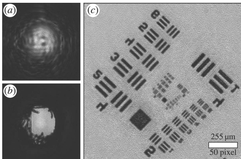
Figure 3. Real and constructed images in ptychography 4
