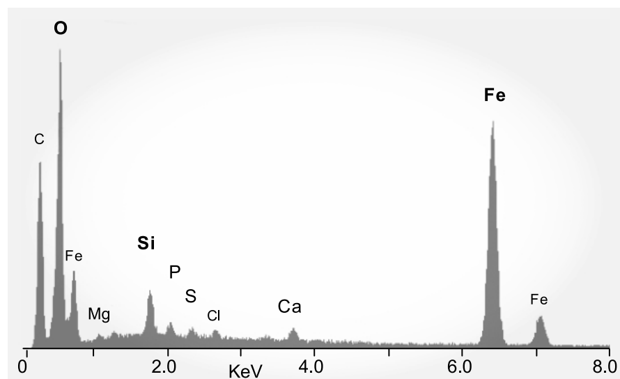
Figure 6. Energy Dispersal X-ray Spectrum (EDS) 10
