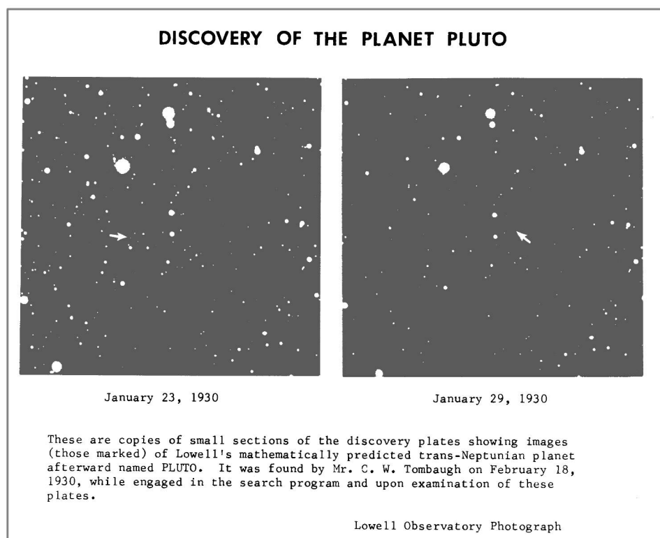
Figure 11. Clyde Tombaugh's images in which Pluto was found 15
