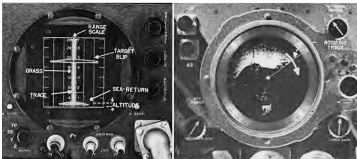
Figure 4. “L-type scope” and “PPI-type scan” in early radar sets 6
