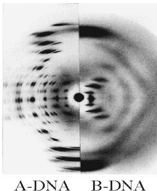
Figure 15. X-ray diffraction patterns for two forms of DNA 20
