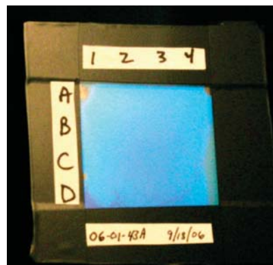
Figure 1. 3 cm \times 3 cm TGCCA fabricated between glass plates by using a 100 \mu m thick polyester spacer to separate the TGCCA from the adhesive used to seal the edges of the glass plates. The cell was divided into 16 9 mm square regions (A1–D4) that were analyzed via UV–vis transmission spectroscopy by using a 5 mm diameter aperture.
