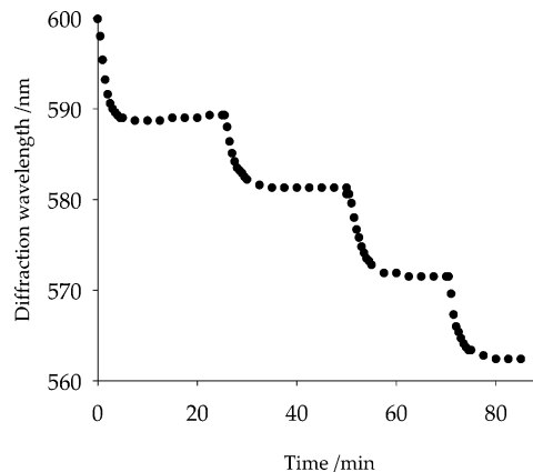
Figure 11. Response kinetics of hexyl acrylate PCCA glucose sensors upon exposure to multiple additions of a freshly prepared 0.2 mM D-glucose solution in 5 mM Gly-Gly buffer, 150 mM NaCl, pH 7.4 at 37 °C. A repeatable rapid blue shift of the diffraction ( \sim 10 \pm 1 nm) is observed saturating within \sim 300 s.
