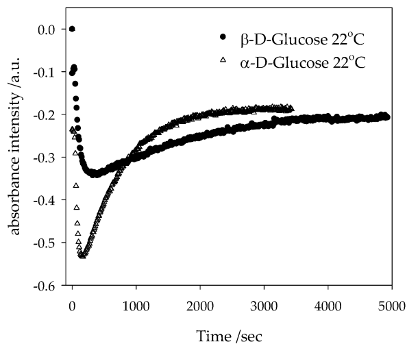
Figure 5. Absorbance changes at 304 nm as function of time after addition of 100 mM freshly prepared \alpha -D-glucose and \beta -D-glucose to 10 mM 5A-2F-PBA Gly-Gly buffer solution at pH 7.4 with 150 mM NaCl at 22 (left) and 37 °C (right). Path length, 2 mm.
