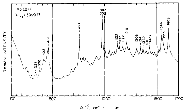
FIGURE 5: Resonance Raman spectrum of Mb III F. \lambda_{\text{ex}} = 5999.7 \text{ \AA} ; heme concentration = 0.27 \text{ mM} ; 0.2 \text{ M Na}_2\text{SO}_4 ; 0.1 \text{ M HEPES} buffer; 0.5 \text{ M NaF} ; pH 6.77; three scans; laser power = 0.5 \text{ W} ; integration time = 1 \text{ s} ; average slit width = 4.1 \text{ cm}^{-1} .
