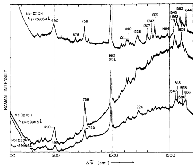
FIGURE 2: Resonance Raman spectra of Mb III OH and Hb III OH. Hb III OH: \lambda_{ex} = 5998.5 \text{ \AA} ; heme concentration = 0.36 mM; 0.2 M Na 2 SO 4 ; 0.02 M borate buffer; pH 10.62; nine scans; laser power = 0.3 W. Mb III OH: heme concentration = 0.31 mM; 0.25 M Na 2 SO 4 ; 0.025 M borate buffer; pH 10.18. \lambda_{ex} = 5998.5 \text{ \AA} ; laser power = 0.3 W; integration time = 1 s; average slit width = 2.7 cm -1 ; one scan. \lambda_{ex} = 5803.4 ; laser power = 0.4 W; integration time = 2 s; average slit width = 2.9 cm -1 ; two scans.
