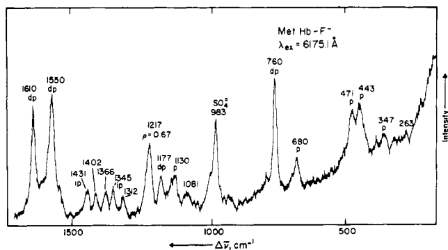
FIGURE 8: Resonance Raman spectrum of MetHb-F - (0.76 mM heme) containing 0.25 M Na 2 SO 4 as an internal standard: λ ex 6175.1 Å; energy 2 \times 10^{-3} J/pulse; pulse repetition rate 30 Hz; scan speed 23 Å/min; slit width 3.7 Å; p, polarized; dp, depolarized; ip, inversely polarized.
