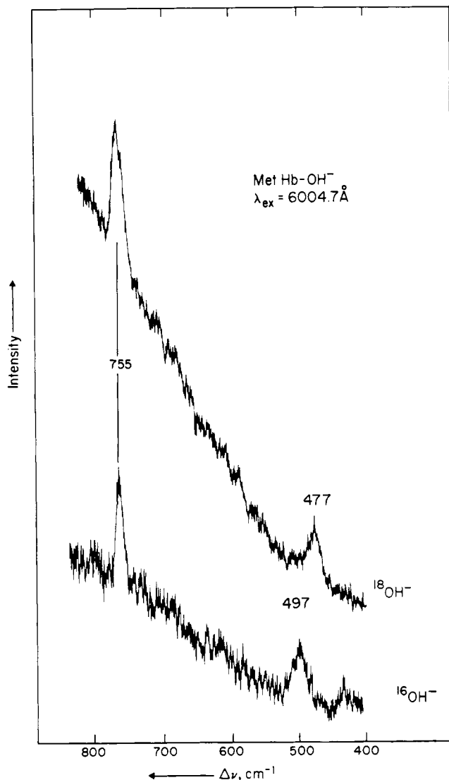
FIGURE 7: Resonance Raman spectra of MetHb- 16 O - and MetHb- 18 O - (ca. 0.9 mM heme): pH 10.2; λ ex 6004.7 Å; energy 2 \times 10^{-3} J/pulse; pulse repetition rate 30 Hz; scan speed 16 Å/min; slit width 4.5 Å.
