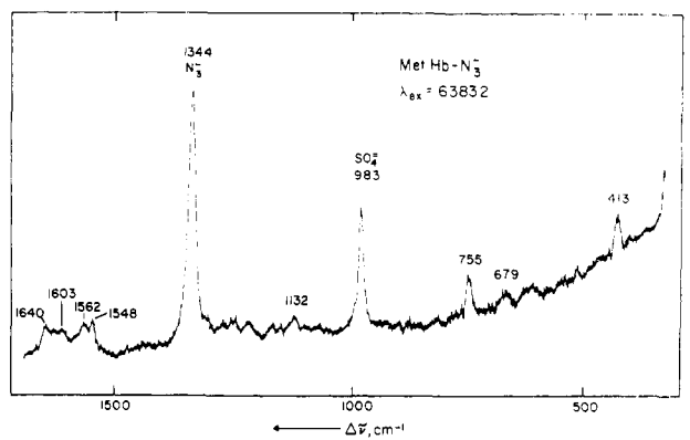
FIGURE 2: Resonance Raman spectrum of MetHb-N 3 - ; λ ex 6383.2 Å; conditions as in Figure 1.
