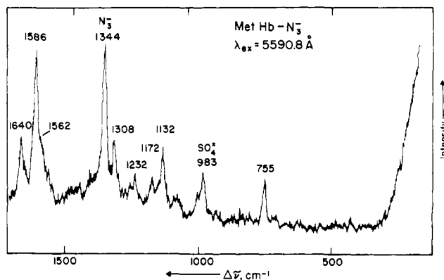
FIGURE 1: Resonance Raman spectrum of MetHb-N 3 - (0.76 mM heme) containing 0.25 M Na 2 SO 4 as an internal standard: λ ex 5590.8 Å; energy 10 -3 J/pulse; pulse repetition rate 30 Hz; scan speed 23 Å/min; slit width 3 Å. Positions of Raman lines due to SO 4 2- and uncomplexed azide are shown in the figure.
