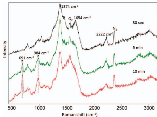
Fig. 8. Here, 229 nm DUVRR spectra of solid-state photolyzed RDX on a SiO 2 substrate with varying irradiation times. The sample was stationary during excitation and contained ~1 mg of RDX. The sample was irradiated with 8.5 mW of a CW 229 nm laser beam focused to a spot size of ~200 μm. The 1555 and 2368 cm -1 bands derive from atmospheric oxygen and nitrogen, respectively.
