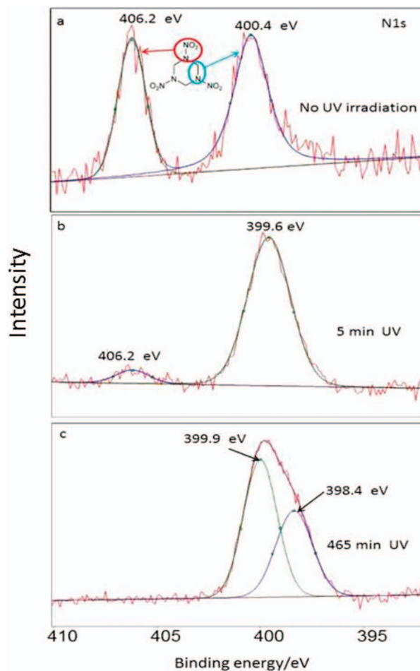
Fig. 9. Nitrogen 1 s electron XPS spectra of RDX (on a gold substrate) at different irradiation times: (a) RDX with no UV irradiation, (b) RDX after 5 min of UV irradiation, and (c) RDX after 465 min of UV irradiation. The spectra were fit to Gaussian bands. The RDX sample was irradiated with 5 mW of a CW 229 nm laser beam focused to a spot size of ~300 μm.
