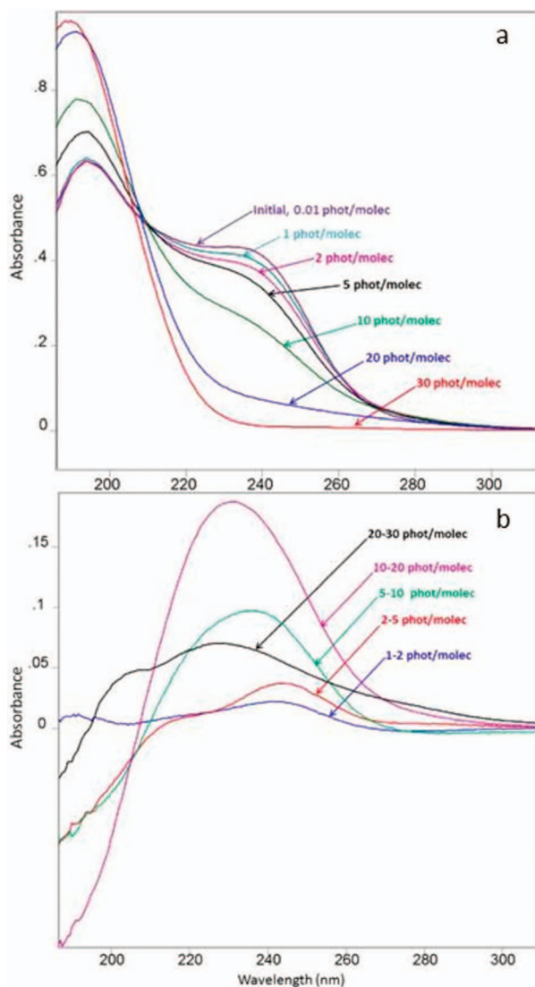
FIG. 2. (a) Dependence of the absorption spectra of RDX in \text{CD}_3\text{CN} upon irradiation of 0.01, 1, 2, 5, 10, 20, and 30 photons per molecule by 229 nm light measured in a 0.05 mm path length cuvette. (b) Absorbance difference spectra between 1–2, 2–5, 5–10, 10–20, and 20–30 photons per molecule absorption.
