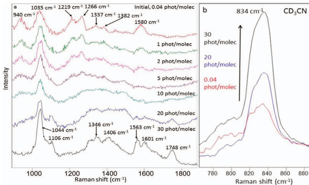
Fig. 1. (a) Solution DUVRR spectra of RDX in \text{CD}_3\text{CN} with increasing irradiation (photons absorbed per molecule). Here, 1 mL of 3 mg/mL RDX in \text{CD}_3\text{CN} was irradiated with 17 mW of 229 nm light. Quartz and \text{CD}_3\text{CN} Raman bands were subtracted. (b) DUVRR spectra of the 834\text{ cm}^{-1} \text{CD}_3\text{CN} band in the RDX spectra with increasing irradiation time. The \text{CD}_3\text{CN} band increases in intensity as the photolysis increases.
