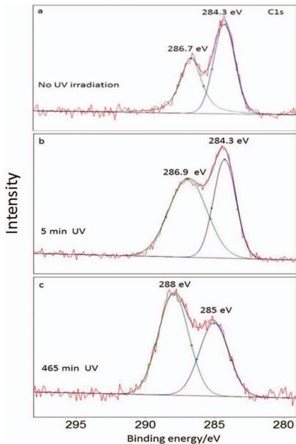
FIG. 10. Carbon 1 s electron XPS spectra of RDX (on a gold substrate) after different irradiation times: (a) RDX without UV irradiation, (b) RDX with 5 min of UV irradiation, and (c) RDX with 465 min of UV irradiation. The spectra were fit to Gaussian bands. The RDX sample was irradiated with 5 mW of a CW 229 nm laser beam focused to a spot size of \sim 300 \mu\text{m} .
