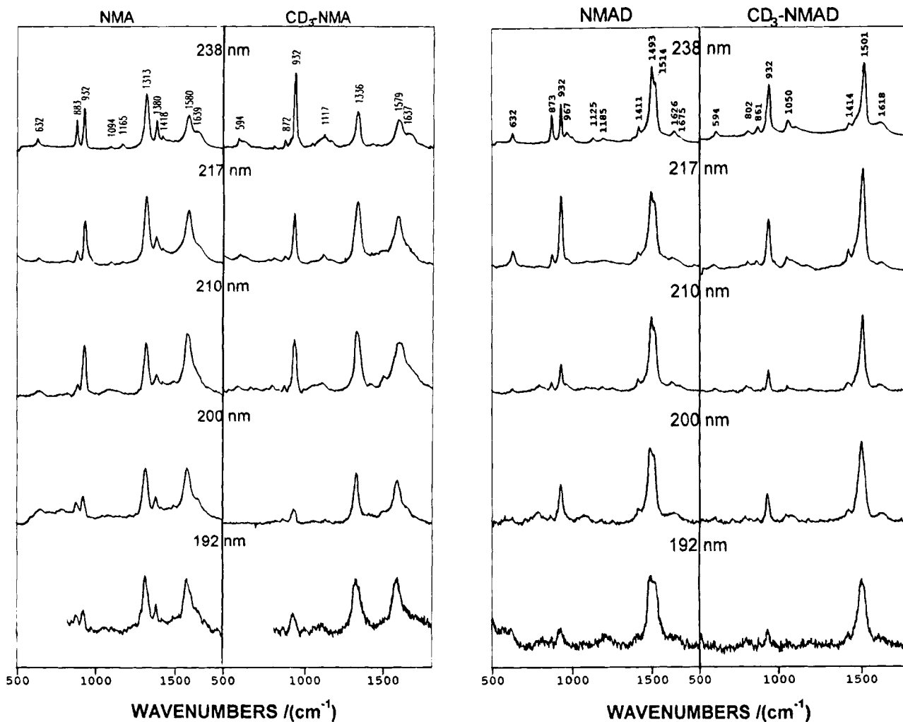
Figure 2. Raman spectra of NMA, CD 3 -NMA, NMAD, and CD 3 -NMAD as function of excitation wavelength. Sample concentrations are as follows. NMA: 194 mM at 238 nm, 49 mM at 217 nm, 9.8 mM at 210 nm, 3.6 mM at 200 nm, and 2.7 mM at 192 nm. CD 3 -NMA: 196 mM at 238 nm, 50 mM at 217 nm, 9.9 mM at 210 nm, 4.2 mM at 200 nm, and 3.0 mM at 192 nm. NMAD: 111 mM at 238 nm, 23 mM at 217 nm, 8.4 mM at 210 nm, 3.0 mM at 200 nm, and 2.7 mM at 192 nm. CD 3 -NMAD: 101 mM at 238 nm, 26 mM at 217 nm, 9.9 mM at 210 nm, 3.1 mM at 200 nm, and 2.6 mM at 192 nm. The 932 cm -1 band derives from ClO 4 - used as an internal standard. ClO 4 - concentration: 1.0 M for CD 3 -NMA at 238 nm and NMAD at 217 nm; 0.3 M for NMAD at 238 nm; 0.5 M for the other spectra. Spectral resolution: ca. 5 cm -1 for 238 nm, 7 cm -1 for 217 nm, 12 cm -1 for 210, 14 cm -1 for 200 nm, 20 cm -1 for 192 nm spectra, respectively. The 238 nm excitation utilized 8 mW CW laser power, and the spectra were accumulated over a period of 6 min. The 217, 200 and 192 nm excited spectra were obtained at a 20 Hz repetition rate using 6 ns pulses with laser pulse energies of ca. 0.35, 0.10, and 0.020 mJ with accumulation times of 6, 20, and 35 min, respectively. The 210 nm spectra were obtained at a 100 Hz repetition rate using 16 ns pulses with laser pulse energies of 0.06 mJ with an accumulation time of 9 min.
