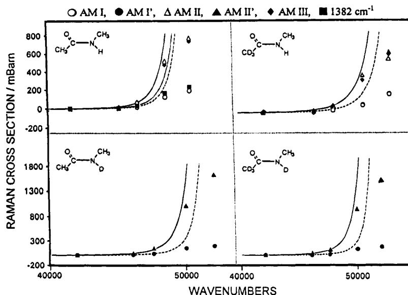
Figure 3. Resonance Raman excitation profiles of NMA, CD 3 -NMA, NMAD, and CD 3 -NMAD. Solid lines correspond to nonlinear least-squares best fits of preresonance data ( \lambda \geq 211 nm) to the Albrecht A-term expression. 12
