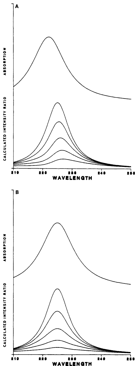
Figure 7. The effect of incident laser power on the measured UVR R excitation profiles. The maximum (true) excitation profile is modeled as a Lorentzian with a bandwidth of ca. 10 nm. The lower excitation profiles were calculated using incident laser powers of 1, 2.5, 5.0, and 10 units, respectively. The absorption spectrum was simulated by using a Lorentzian line shape with a ca. 14-nm bandwidth and a molar absorptivity of 9000 \text{ M}^{-1} \text{ cm}^{-1} . (A) Effect of increase in laser power on an excitation profile which is shifted with respect to the absorption band. (B) Effect of increase in laser power on an excitation profile whose maximum is coincident with that of the absorption band.
