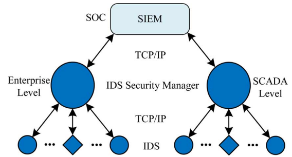
Fig. 2. SCADA-IDS security-management system.
