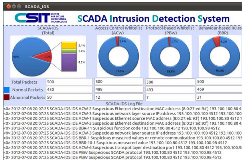
Fig. 6. GUI for displaying SCADA-IDS detection results.
