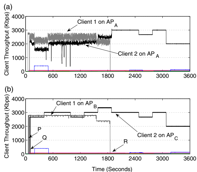
Figure 12 Time series plot of the throughput received by the clients during the heavy traffic load 1-h interval, a without SEAR's load diversion mechanism, and b with SEAR's load diversion mechanism
