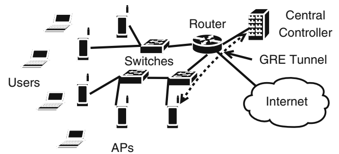
Figure 1 A centralized WLAN infrastructure
