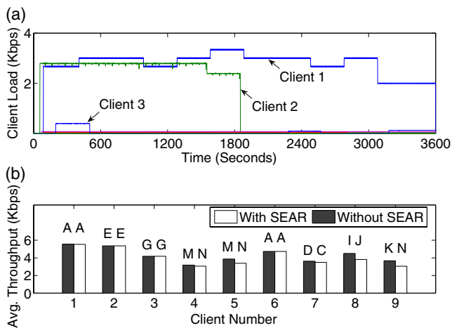
Figure 9 a Nine clients’ load in a 15 AP WLAN. b Average throughput received by the nine clients, without and with SEAR
