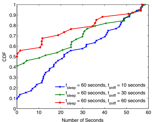
Figure 7 CDF of wait times experienced by APs when t_{sleep} = 60 s, and t_{sniff} is 10, 30, and 60 s. The percentage energy savings for the three sets are 71.2%, 57%, and 43%, respectively
