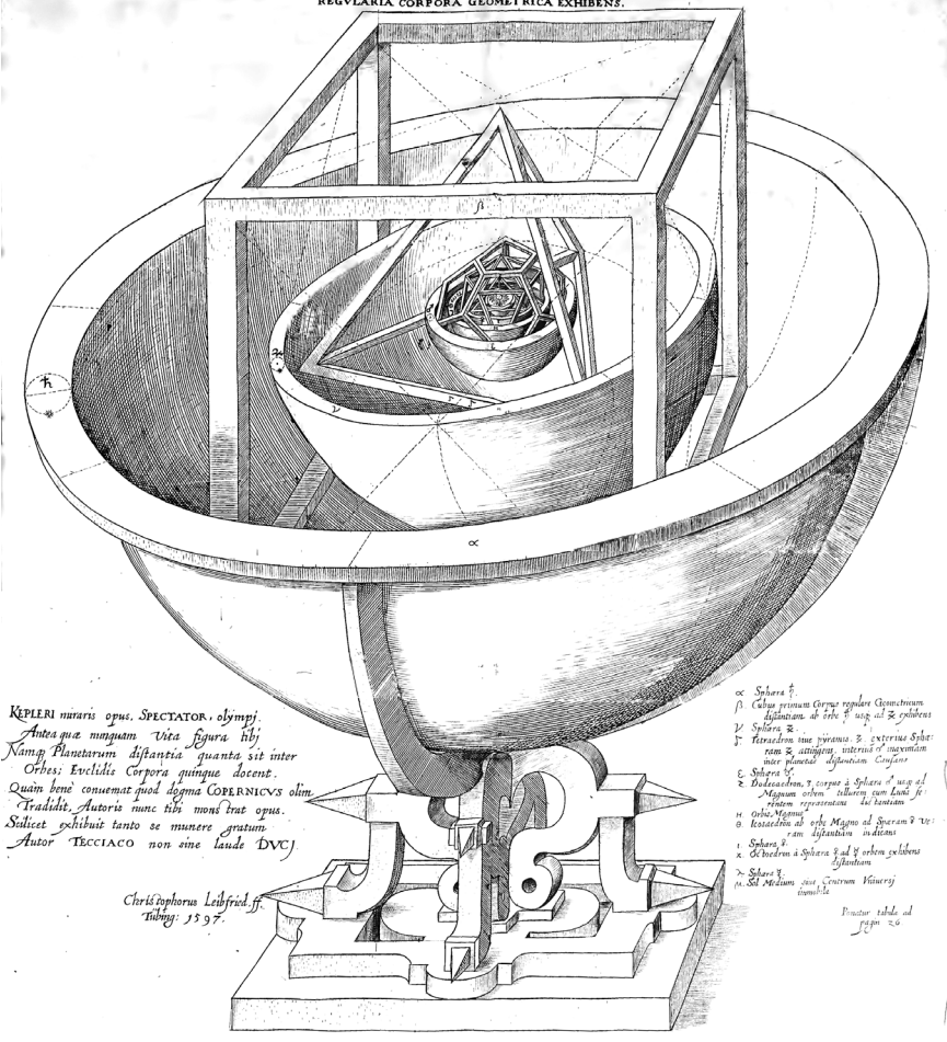
Figure 12.7. Kepler's construction
