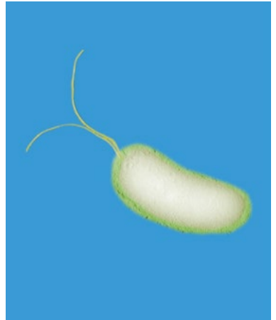
Electron micrograph of a bacterium with hair-like flagella.
