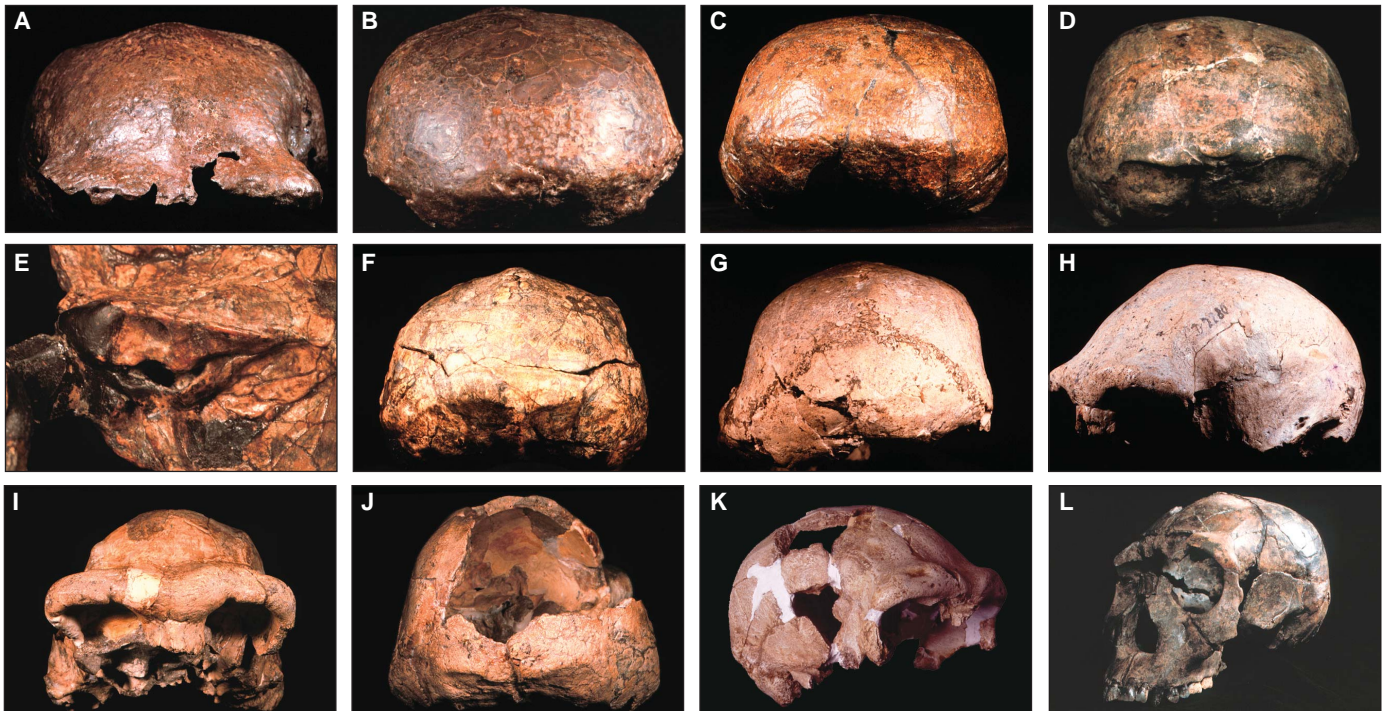
The skull beneath the skin. Various specimens attributed to Homo erectus . The Trinil fossils (the H. erectus type specimen) and the Sangiran fossils represent the same species and show a wide range of individual variation. Note the odd shape of Trinil and Sangiran rear profiles, variation between individuals, and differences between these specimens and various specimens from Africa and Eurasia (G–L). (A and B) Trinil skull cap (front and rear views). (C) Sangiran 2 (rear view). (D) Sangiran 12 (rear
