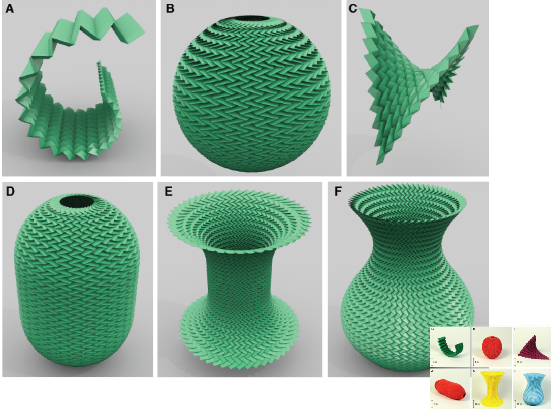
FIGURE 12. While this paper has focused on surfaces with varying degree of smoothness, an interesting new avenue for exploration is that of discrete surfaces [41] that have strongly creased regions, seen for example in Origami.
