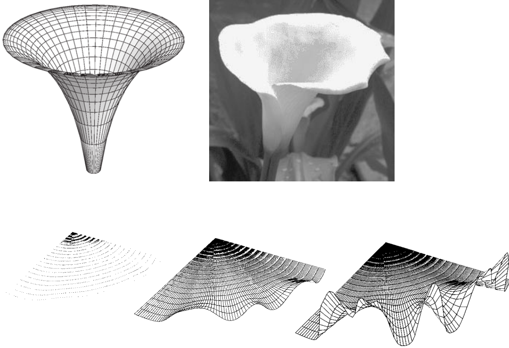
FIGURE 8. (a) Pseudosphere. (b) Picture of a calla lily. (c) Sample plots of the Jacobian function, encoding the Gauss curvature of the prestrain [104].
