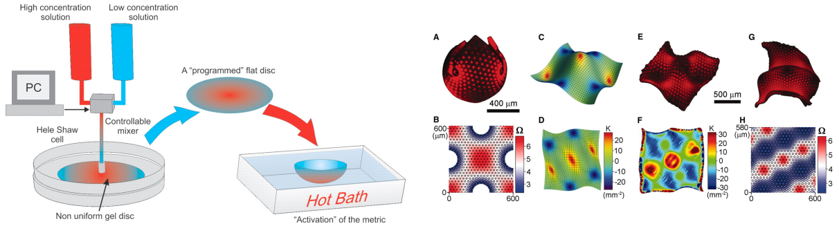
FIGURE 4. Imposing nontrivial target metrics in sheets of NIPA gels. The figures shown are: (a) radially symmetric discs cast by injecting the solution into the gap between two flat glass plates through a central hole [68, Reprinted with permission from AAAS], (b) nonaxisymmetric swelling patterns constructed by half-tone gel lithography in [67, Reprinted with permission from AAAS].
