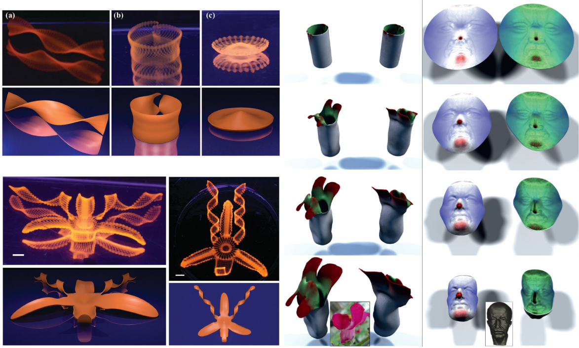
FIGURE 11. Examples of solutions of inverse problems in morphogenesis - to program the metric structure and thence create complex shapes from flat sheets. On the left [50] are shown experiments with 3d printed gel structures that swell in a good solvent, along with representative numerical solutions that are based on minimizing the energy (4.1). On the right [125, Copyright (2021) National Academy of Sciences] we see results of the solution of inverse problems to grow a flower from a bilayer cylindrical shell, and a face from a circular bilayer disk.
