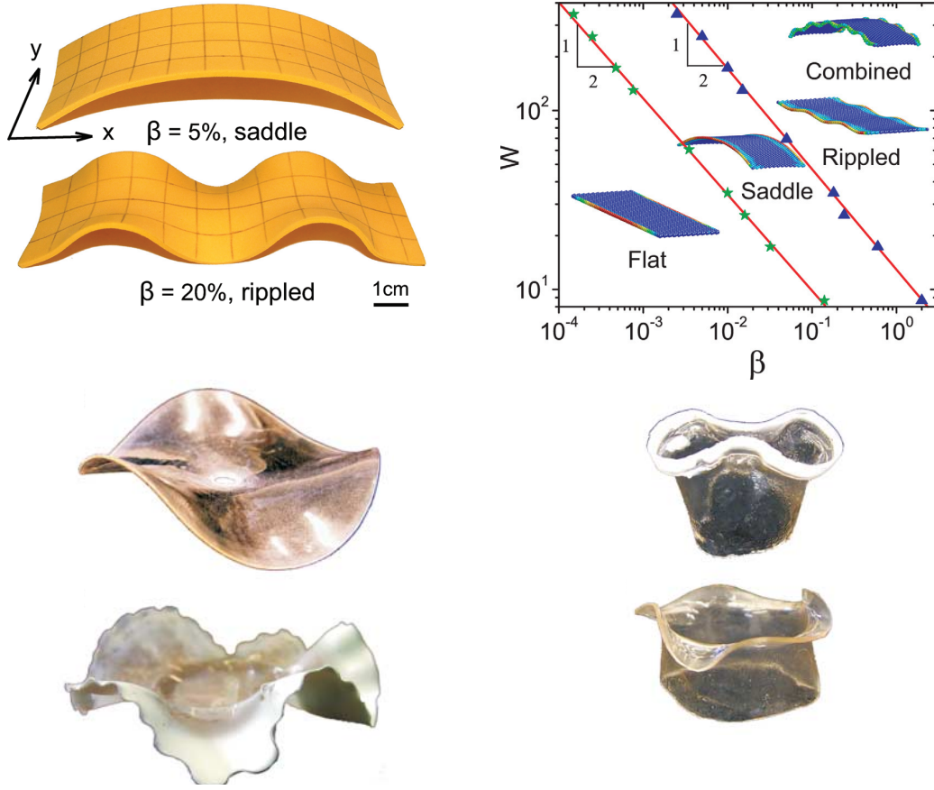
FIGURE 6. A range of patterns arise when a thin sheet is inhomogeneously stretched plastically or swells in response to a solvent. (a) By dragging one's nails along the edges of a foam strip weakly, a flat surface transitions to one that is hyperbolic. (b) The same process carried out strongly leads to a surface that is strongly rippled, much like the edges of a leaf [93, Copyright (2021) National Academy of Sciences]. (c) Thin sheets of a circular gel disk deform into a hyperbolic surface with two lobes. (d) Thinner sheets deform into multi-lobed sheets which are able to relieve the swelling-induced frustration by changing their curvature on multiple scales [68, Reprinted with permission from AAAS].
