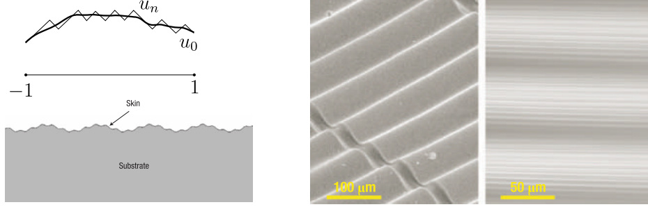
FIGURE 3. (a) A short map approximation of u_0 (darker line) by a zigzag u_n with u'_n = \pm 1 . (b) A computational realization of hierarchical wrinkles that arise when a thin stiff film is coated atop a soft substrate and the system is then subject to a reduction in temperature that leads to differential shrinkage [42]. (c) An experimental realization of the hierarchical wrinkles that shows two (of a total of six) generations of wrinkles. The three examples serve to link convex integration to models and experiments in materials science [42].
