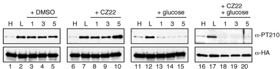
FIGURE 5. Activity of the Glc7-Reg1 phosphatase is regulated by glucose. Cells expressing the analogue sensitive Tos3-L135G protein as the only SAK were grown in high glucose media ( H ) and then shifted to low glucose ( L ) for 30 min. Me 2 SO ( DMSO ), CZ22 dissolved in Me 2 SO, or glucose was added, and aliquots were removed after 1, 3, or 5 min. Extracts were prepared, and the HA-tagged Snf1 protein was collected by immunoprecipitation and analyzed by Western blotting using antibodies directed against the phosphorylated form of the Snf1 activation loop (α-PT210) or against total Snf1 protein (α-HA).
