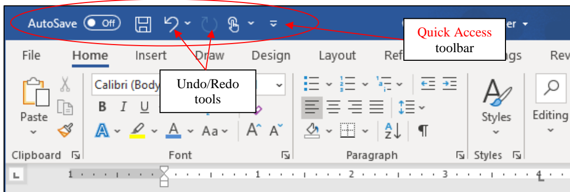
Fig. 1.24 Undo/Redo tools
