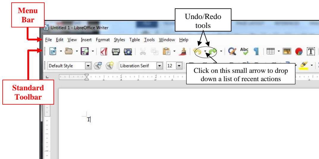
Fig. 1.7 Undo/Redo tools
