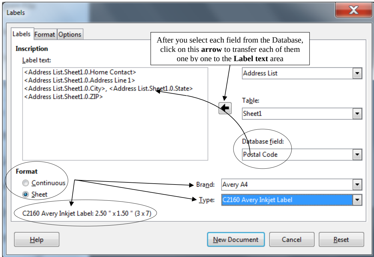
Fig. 7.17 The Labels dialog box after filling out the various entries
