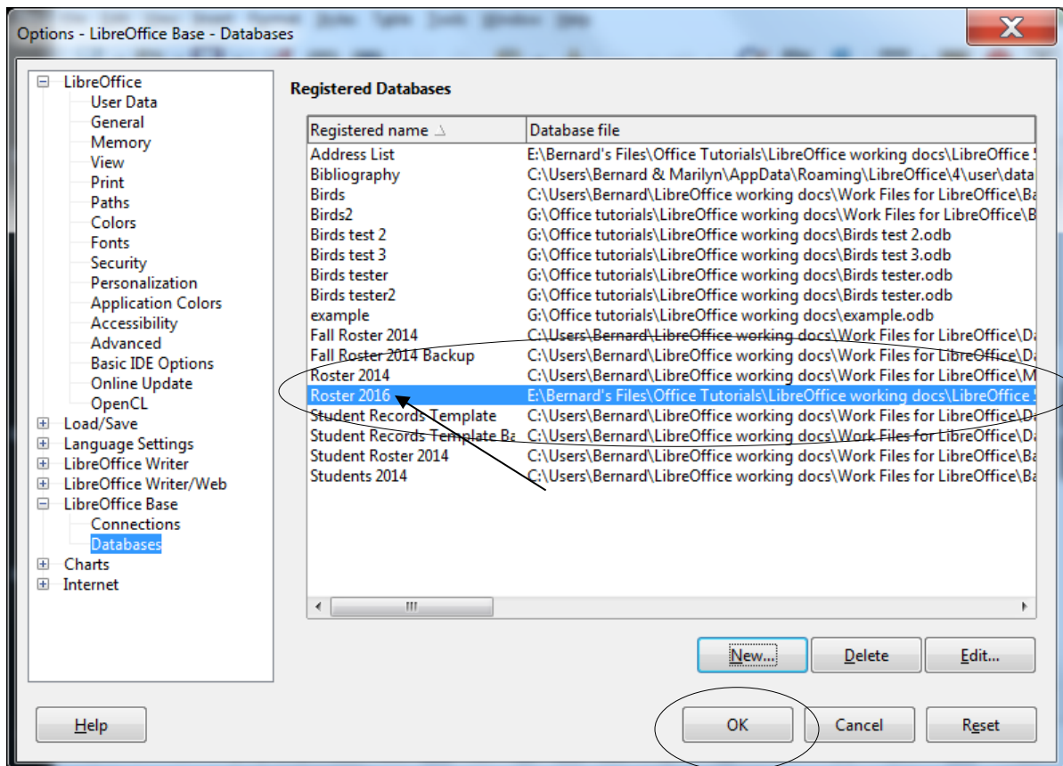
Fig. 7.25 Adding Roster 2016 to the list of registered databases
