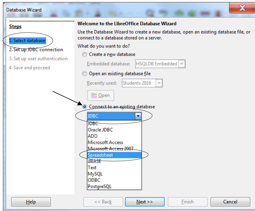
Fig. 7.4 The LibreOffice Database Wizard
