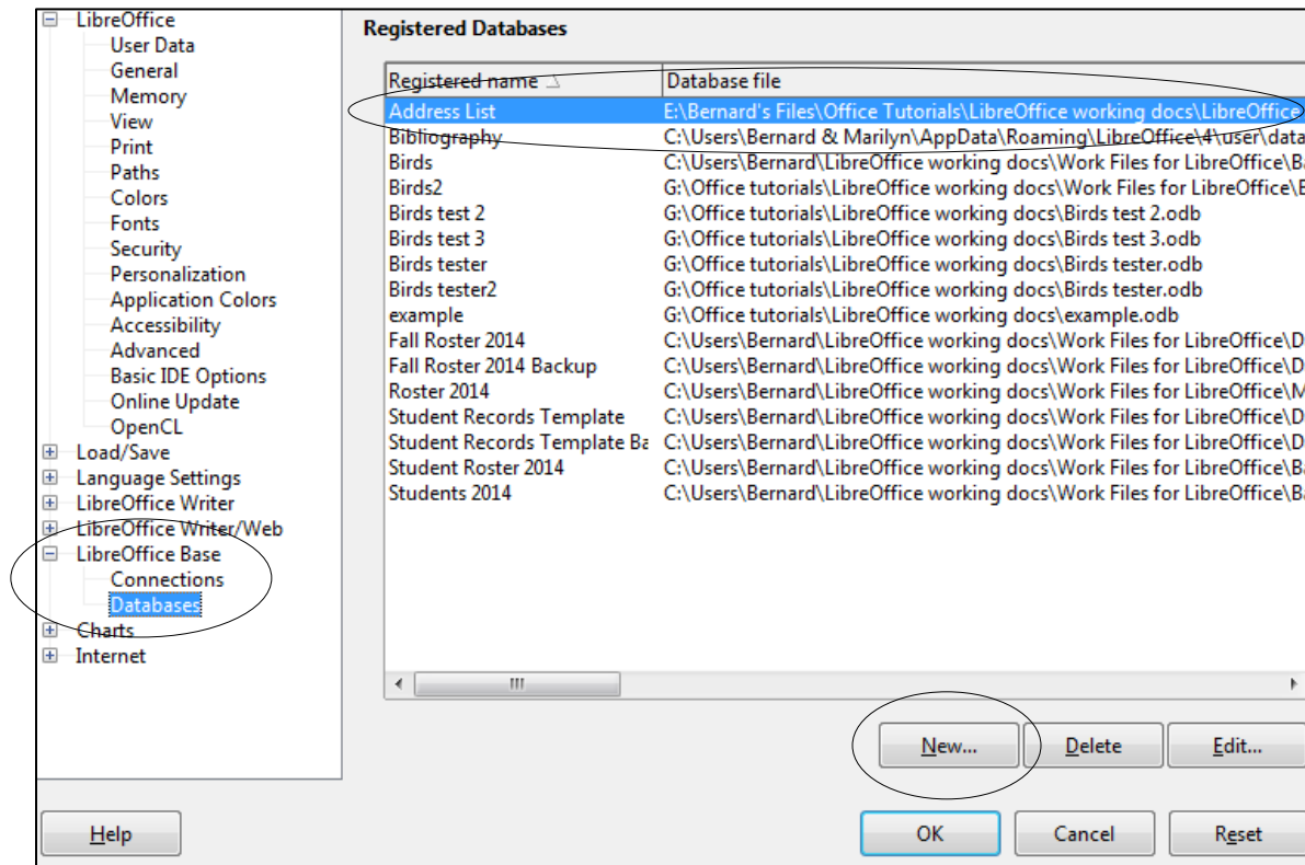
Fig. 7.23 The Tools > Options > LibreOffice Base – Databases dialog box
