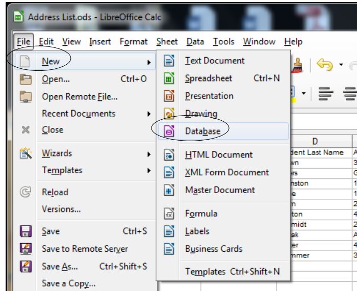
Fig. 7.3 Opening a new database
