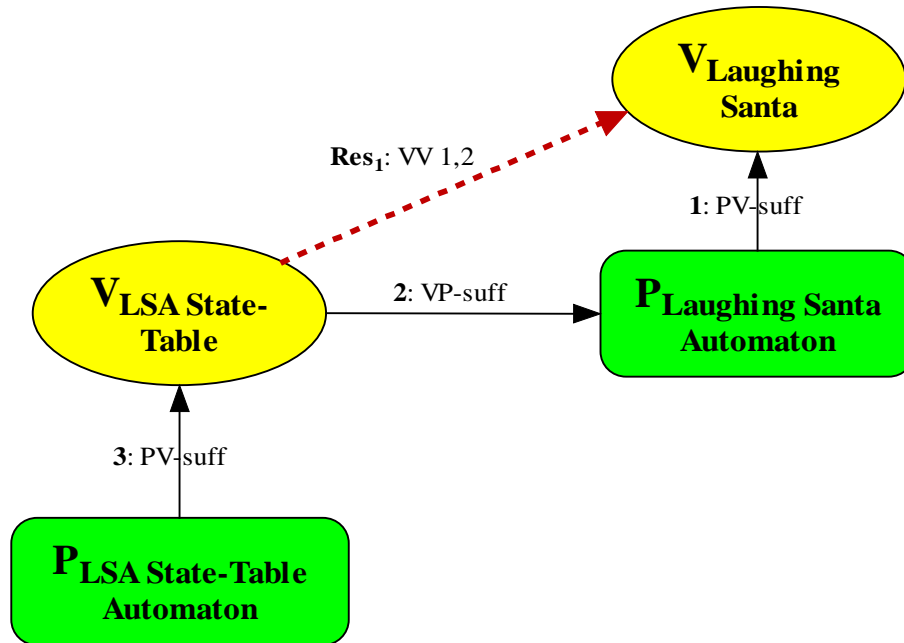
Meaning-Use Diagram #6: Specifying the Automaton that Deploys the Laughing Santa Vocabulary
