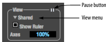
Figure 10-10: View controls.
