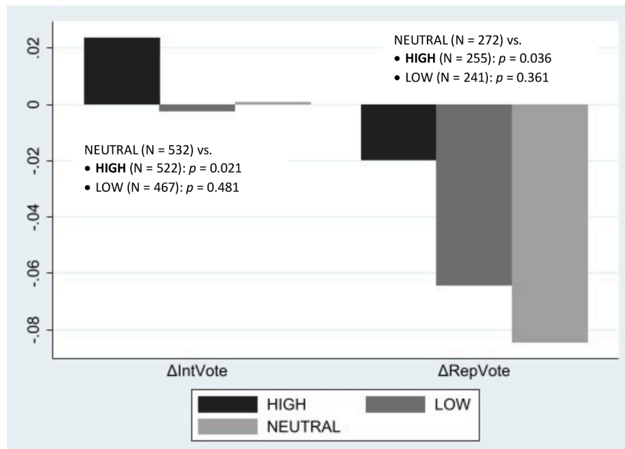
Fig. 2. Effect of HIGH and LOW treatments on voting Notes: Figure shows effect of treatment on intended / reported voting relative to PriorAttitude (-1 is ‘certainly against’ to 1 ‘certainly in favor’). \Delta IntVote is the normalized [-1,1] difference between intended voting reported at the end of wave 1 and PriorAttitude : \Delta IntVote = [(IntVoting - 3) / 2 - PriorAttitude] / 2 . \Delta RepVote is the normalized [-1,1] difference between self-reported actual voting reported in wave 2 and PriorAttitude : \Delta RepVote = RepVoting - (PriorAttitude - 1) / 6 . Fig. 2 is based on samples who reported the respective outcome variable ( \Delta IntVote : 1,521; \Delta RepVote : 768, respectively, see Table 2). p-values for Mann-Whitney tests against NEUTRAL.
